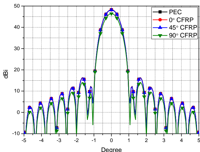
Fig. 4. The radiation pattern according to the laminating directions of the newly proposed material and ideally perfect electric conductor. PEC = perfect electric conductor, CFRP = carbon fiber reinforced polymer.
